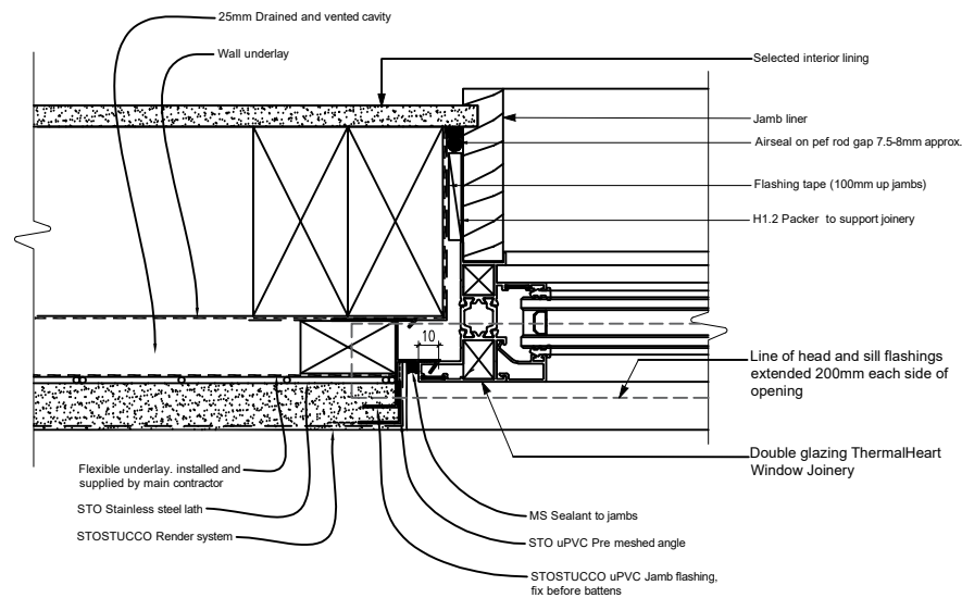
Window Jamb Detail - Plaster Cladding
