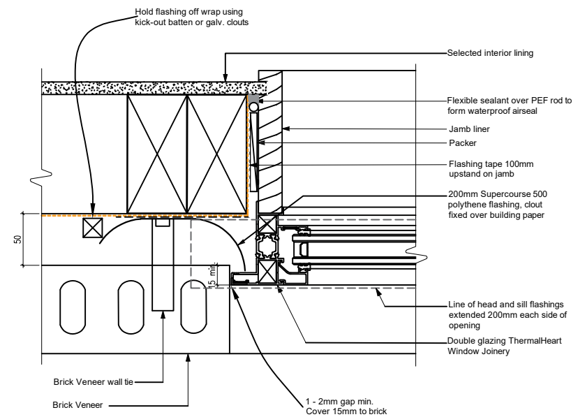
Window Jamb Detail - Brick Veneer Cladding
