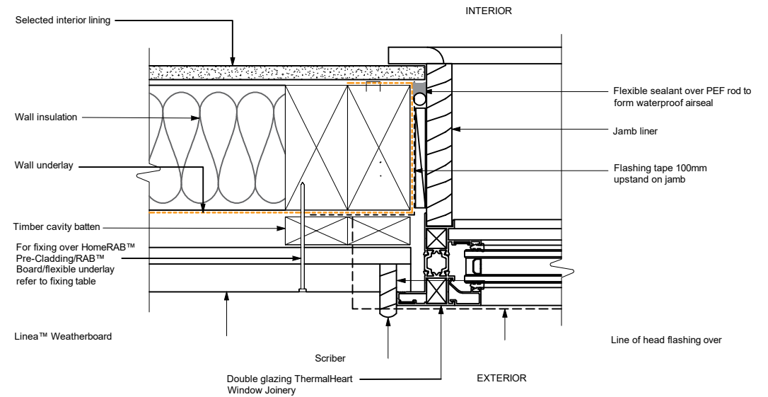
Window Jamb Detail - Weatherboard Cladding with Cavity
